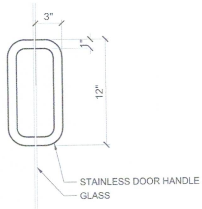
HANDLE DETAILS
