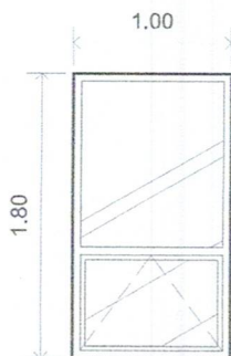
2 SETS AWNING WINDOW
