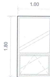
3 SETS AWNING WINDOW
